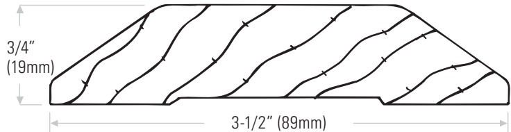
DS3530AK Oak threshold
