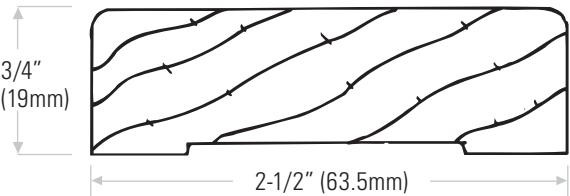
DS2230AK Oak threshold
