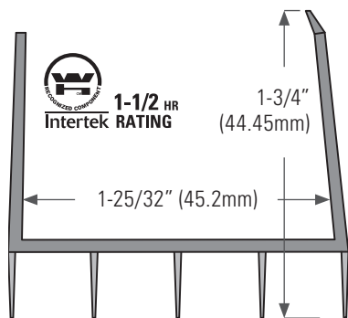
DS127B PVC brown. 36", 48" DS127W PVC white. 32", 36", 48"
