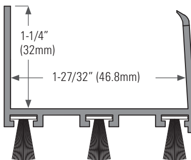
DS125B PVC brown. Lengths available: 36", 48" DS125W PVC white. 32", 36", 48"
