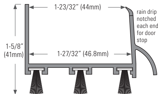
DS124BL PVC black. 35-3/4", 36", 48" DS124B PVC brown. 32", 36", 48" DS124W PVC white. 31-3/4", 32", 35-3/4", 36", 48"
