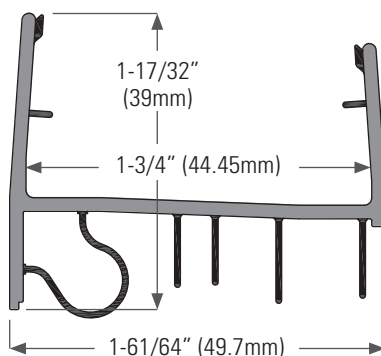
DS232B PVC brown. Lengths available: 36", 48" DS232W PVC white. 31-3/4", 33-3/4", 35-3/4", 48" DS232 door shoe designed for DS458 & DS658 Series sills only
