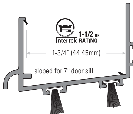
DS2702B PVC brown. Length available: 36" only DS2702W PVC white. Length available: 36" only
