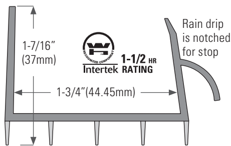
DS128BL PVC black. 32", 35-3/4", 36", 48" DS128B PVC brown. 31-3/4", 32", 35-3/4", 36", 48" DS128W PVC white. 31-3/4", 32", 35-3/4", 36", 48"
