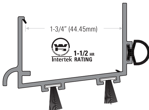
DS2700B PVC brown. Length available: 36" only DS2700W PVC white. Length available: 36" only
