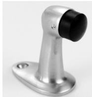
DJ1452 Door Stop Fastener: W/S & Exp. Shield 2 3/4" Projection 2 1/4" x 1 1/4" Base
