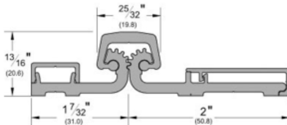
Full Surface Center Pivot 83" PECFS83CP PEDFS83CP PECFS83CP-HD1 PEDFS83CP-HD1
