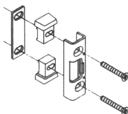
AR 91-0993 8800 Strike Kit For center hung doors with 4" jam
