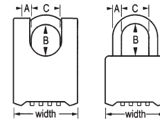
Shackle Dimensions
