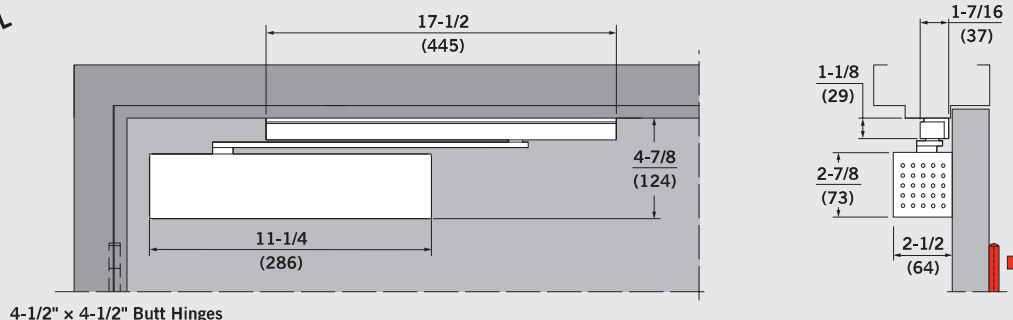
4-1/2" × 4-1/2" Butt Hinges
