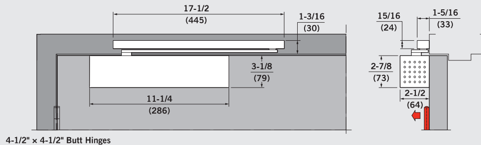
4-1/2" × 4-1/2" Butt Hinges
