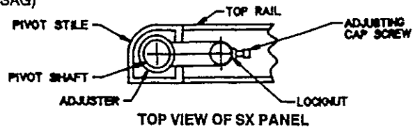
TOP VIEW OF SX PANEL
