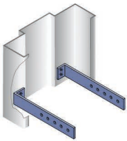
A1 Standard Strap Anchor
