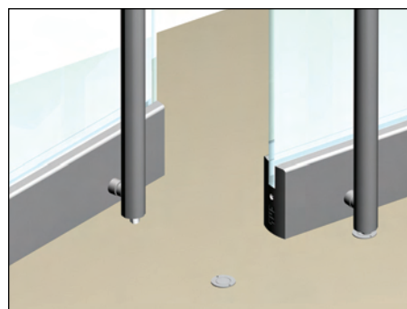
Rail Mount Detail at Latch at Floor With AMR209PS Dust Proof Keeper
