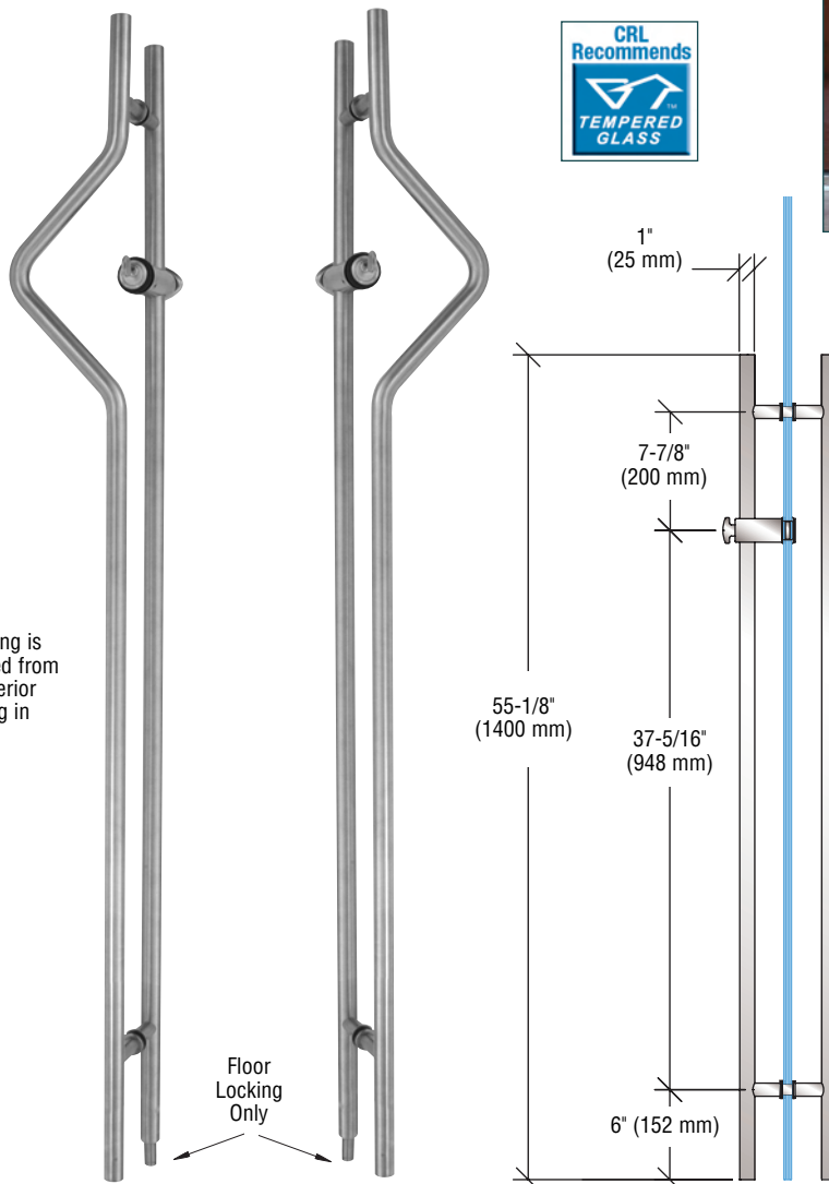
Single Door Installation With Right Hand Locking Handle
