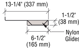
Tray Side View
