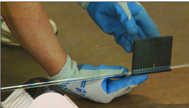
Installing the L-Pressure Block on the Bottom Edge of the Panel and Setting the Panel in the Base Shoe
