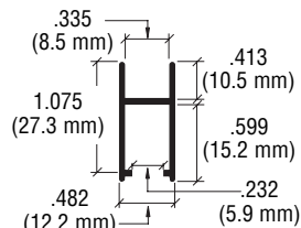
Continental Security Track Assembly shown with Anti-Lift Clip installed
