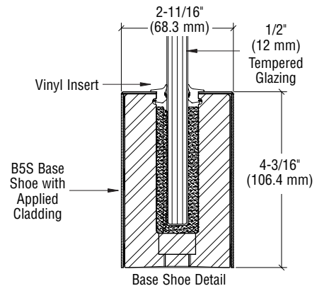
Base Shoe Detail
