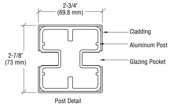
Post Detail
