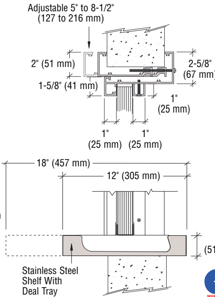
Shown With Optional Cat. No. N666 Speak-Thru and 12" (305 mm) Shelf
