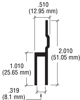
D40 Front Hanger
