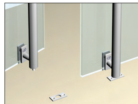
Glass Mount Detail at Latch at Floor With 777SP Flat Strike
