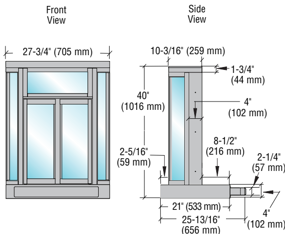
Projected Semi-Automatic Model (Viewed from Clerk Side)
