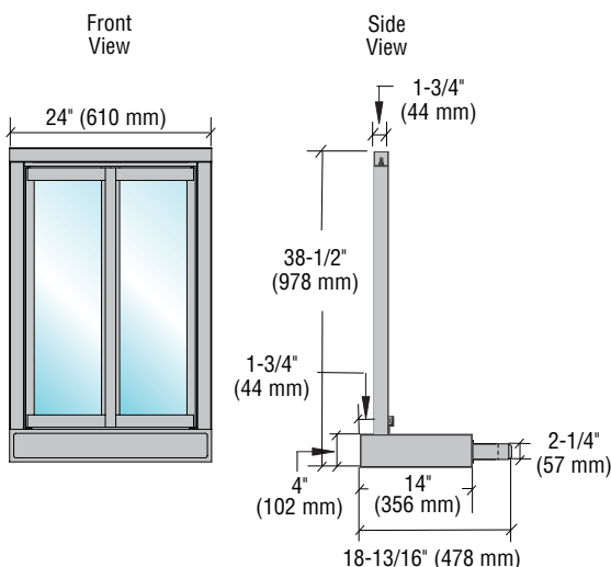
Flush Mount Semi-Automatic Model (Viewed from Clerk Side)
