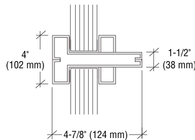
Mullion Detail
