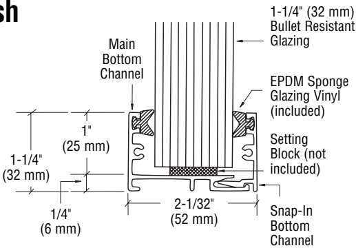
Typical Bullet Resistant Vision Window with Snap Together Sash
