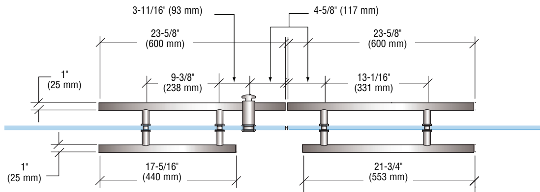
CAT. NO. LLP024BS Brushed Stainless Steel Horizontal Locking Pull Handle
