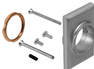
CRL Jackson® #86 Cylinder Mounting Pads
