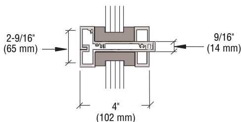
Mullion Detail
