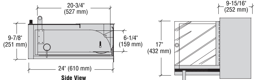
In-Counter Mount Shown
