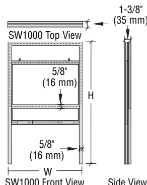
SERIES 1000 NO SCREEN 1-3/8" (35 mm) Frame
