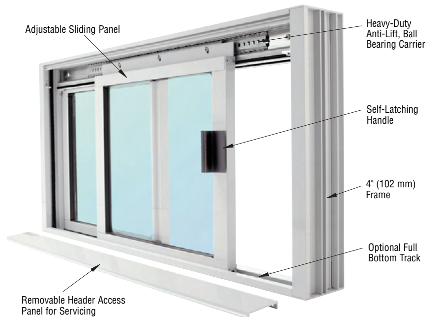
CAT. NO. DW1800A (Shown with Header Access Panel Removed)
