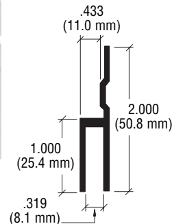
D41 Rear Hanger
