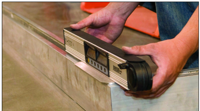
Leveling the Base Shoe Using Our PAL1K Plumb/Angle/Level Locator Kit
