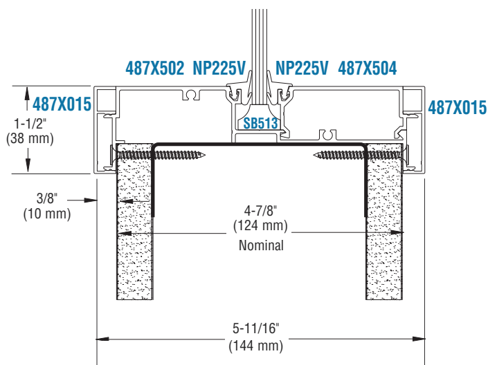
⑫ Borrowed Lite Sill
