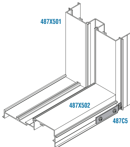
Offset Clip Cat. No. 487C5 (Two Required)
