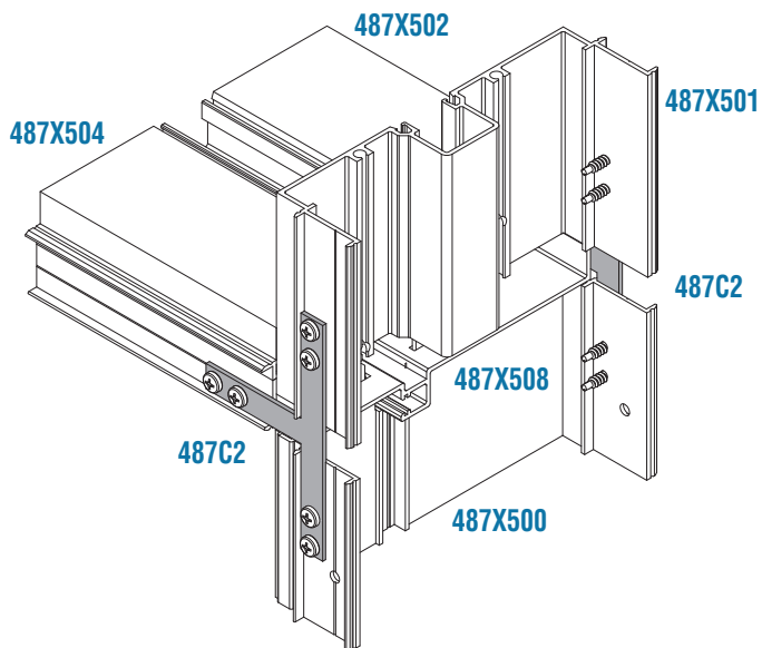
T-Clip Cat. No. 487C2 (Two Required)
