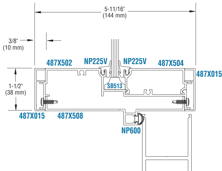
⑤ Door Header with Transom
