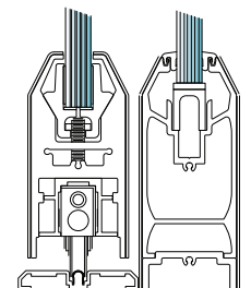
Typical Section of SSR System
