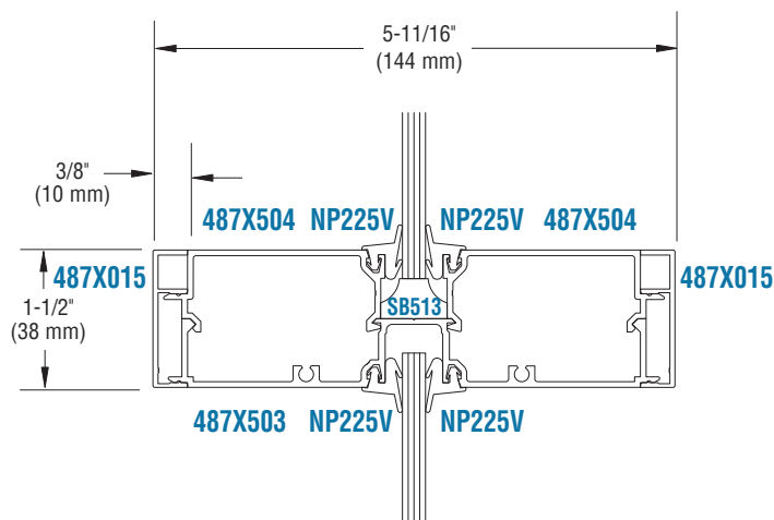
⑩ Intermediate Horizontal
