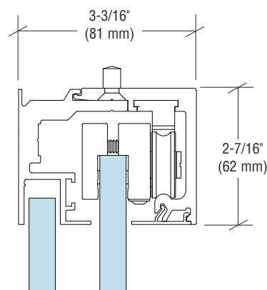
Single Slider With Fixed Panel Kits
