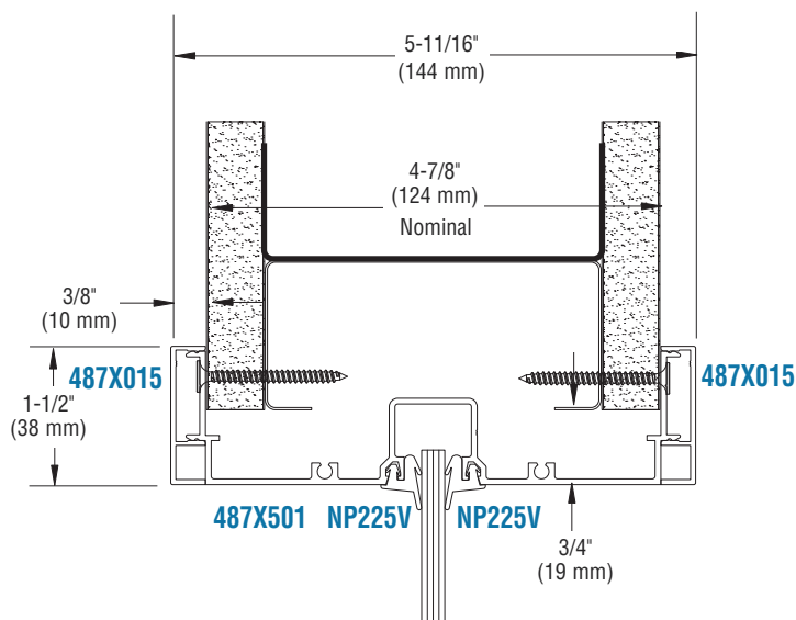
⑨ Fixed Glazing Header
