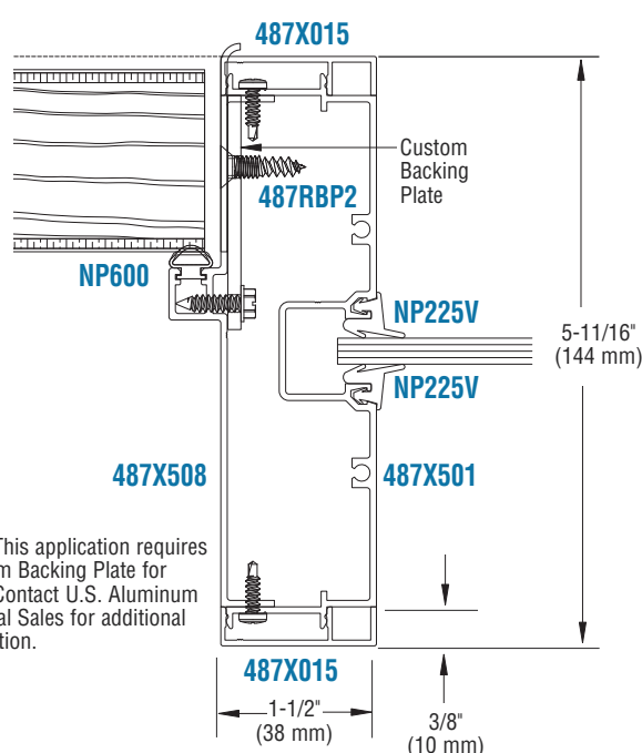
④ Strike Jamb with Sidelite/Transom
