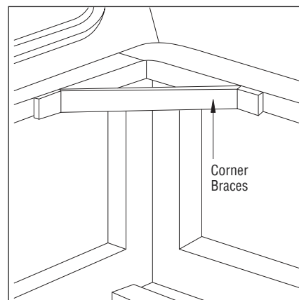
BOX FRONT CORNER BRACES
