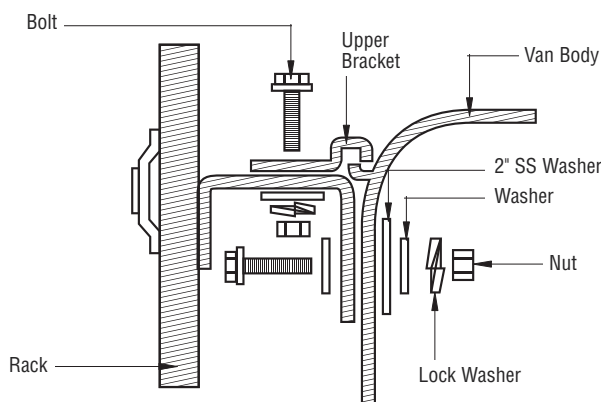
TOP MOUNT
