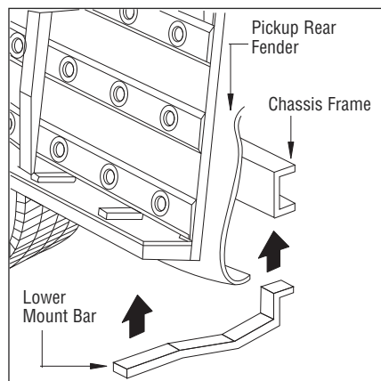
CHASSIS TO RACK MOUNT BARS
