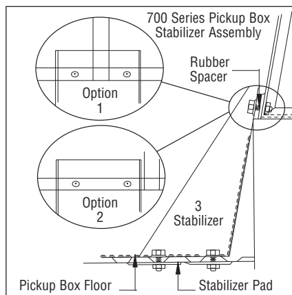
NEW REAR BOX STABILIZERS
