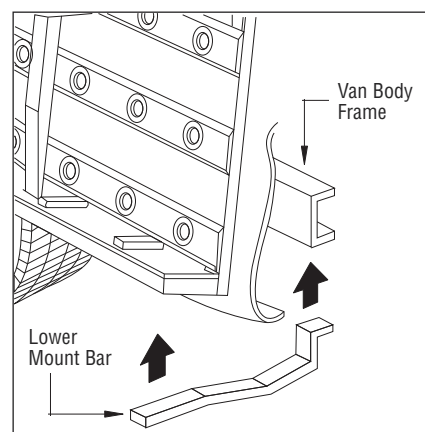
BOTTOM MOUNT
