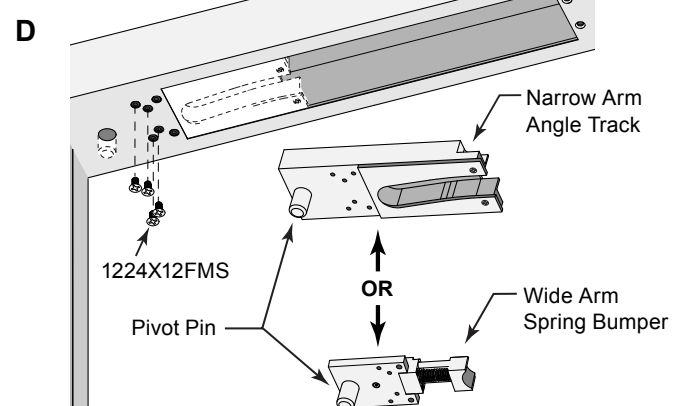
TOP HINGE PIVOT ASSEMBLY
