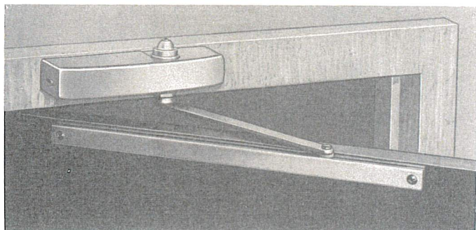
Shown mounted on Frame Minimum Frame required: 3 in.
