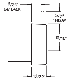
CB-280 TYPE 280 CYLINDER BODY
