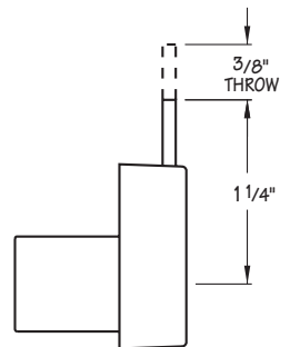
CB-281 TYPE 281 CYLINDER BODY
