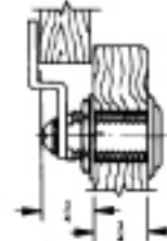
Thick door/drawer construction using NLC8073 with NLC7014-2C cam (sold separately)
