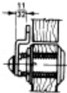
Flush construction with provided formed cam
