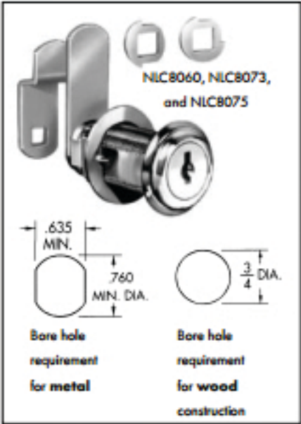
Flush construction with provided formed cam
