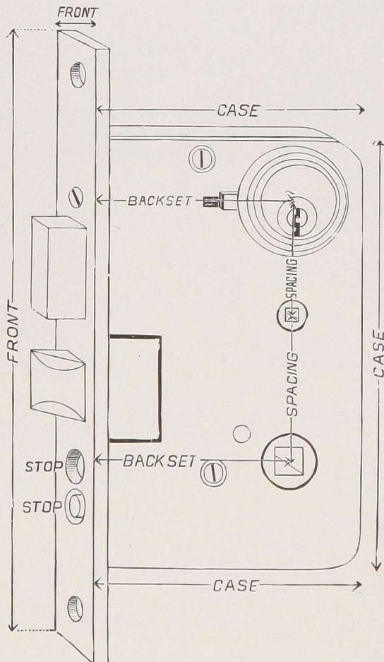
CYLINDER FRONT DOOR LOCK
