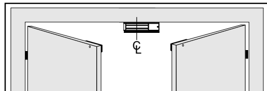
8310 Split Armature Installation
