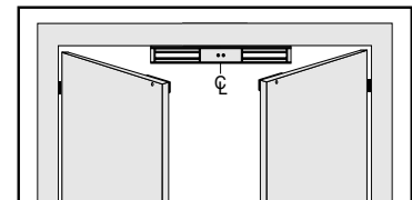
8320 Typical Installation
