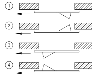
LH SLIDE SWING PLANS
