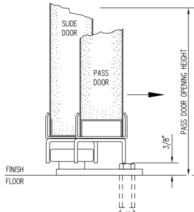
B PASS DOOR SILL SECTION
