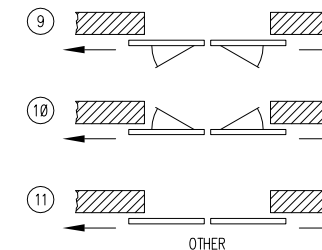
CENTER PARTING SWING PLANS
