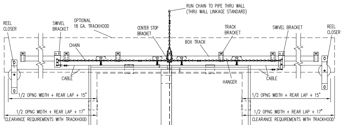
REEL CLOSING SYSTEM
