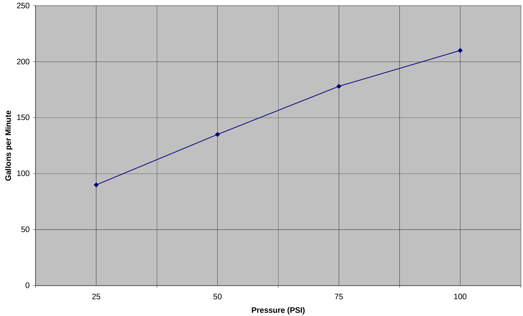
Model 25 Nozzle
