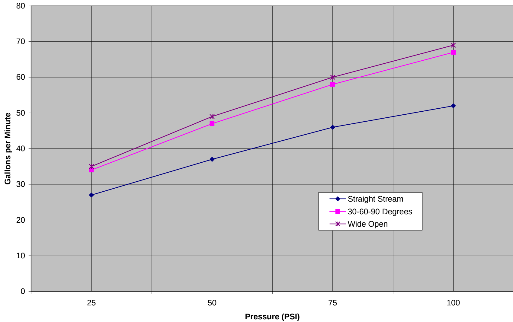
Model 15 Nozzle
