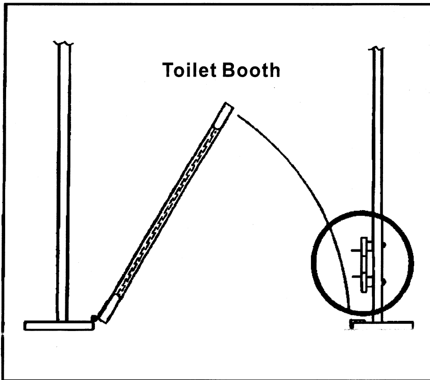
TOILET BOOTH INSTALLATIONS (NO SCALE)
