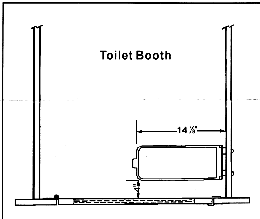
TOILET BOOTH INSTALLATIONS (NO SCALE)
