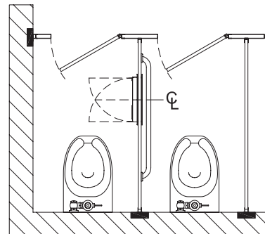
5900 Series Combination Units are to be installed so that doors open 90° to fill product maintain waste container.
