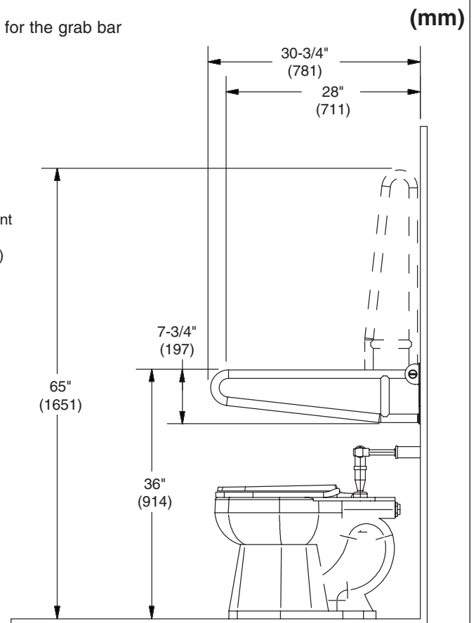
8370-107 Side View
