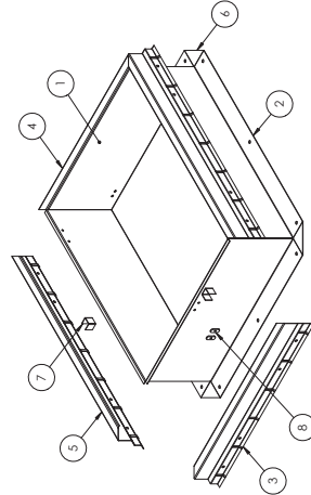
FRAME PARTS
