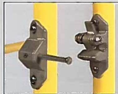
Stainless steel automatic gate latching mechanism patent pending
