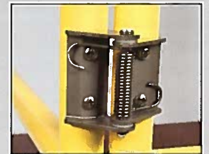
Stainless steel spring hinges and self-closing gate
