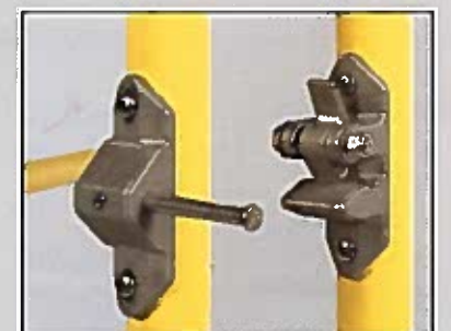
Stainless steel automatic gate latching mechanism patent pending
