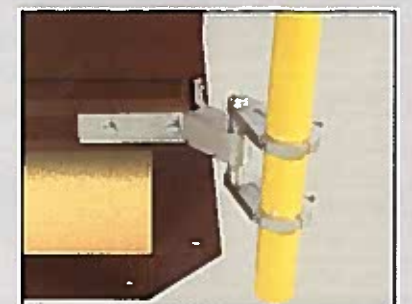
Pivoting post mounting bracket
