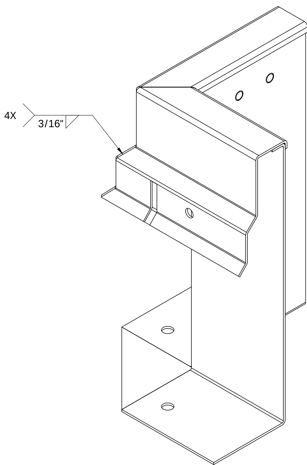
DETAIL G
