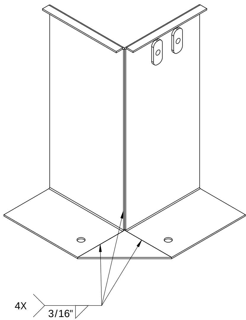
DETAIL C
