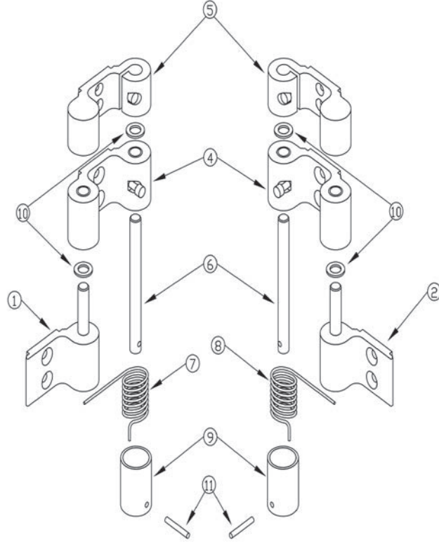
LEFT AND RIGHT IN FOLD READY FOLD UPPER HINGE ASSEMBLY
