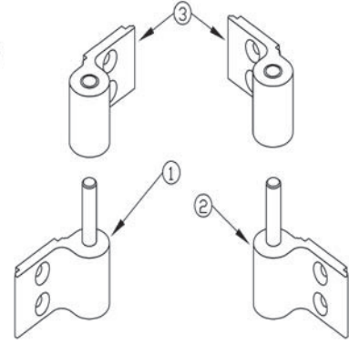
LEFT AND RIGHT IN/OUT FOLD READY FOLD LOWER HINGE ASSEMBLY
