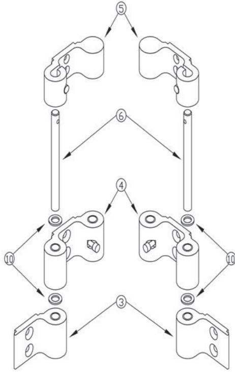
LEFT AND RIGHT OUT FOLD READY FOLD UPPER HINGE ASSEMBLY
