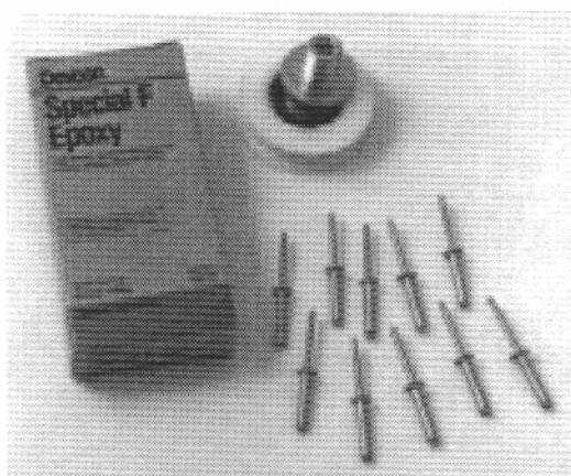
Item #: 11 Track Repair Kit - Part# 11-15-111S Items available separately: Track - Part # 11-01-150S Wheel - Part #:11-04-856S Special "F" Epoxy - Part # 11-20-213S Pop Rivet - Part # 11-09-302S
