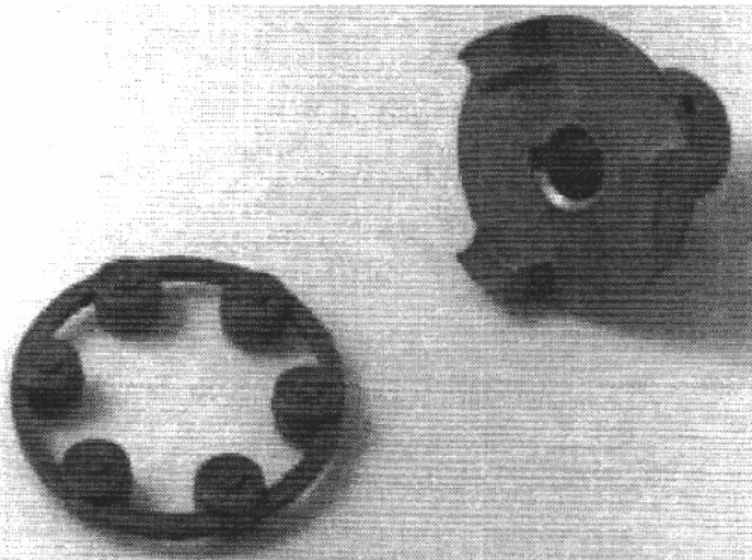
Item #: 1 Drive Arm with Spider, Part # 11-04-180S Rubber Coupling Spider, Part # 10-20-001S
