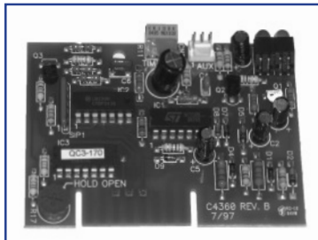
HC43600 Timer Control, DAU, for C4160
