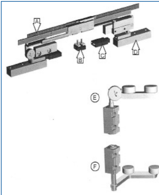
Door Carrier Centre - Items B thru F are detailed on previous page 5.
