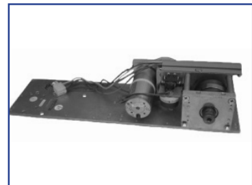
HC7100LI48RB Operator, LH, Inswing, 48 Tooth, Rebuilt
