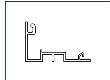
US01-0935-LLCL Redesigned Transom Header Gutter
