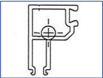
US01-1604-LLCL Non-impact Snap, CL
