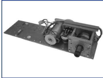
HC7600LI14 Operator, LH, Bi-fold, Inswing, 14 Tooth, Rebuilt
