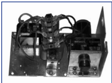
N4420300007 Control, Mercury Relay, CO6/CO8/TM8, Open Chassis, RH, Rebuilt
