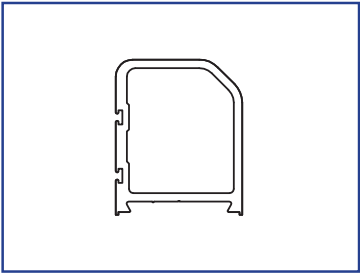
US01-0405-LLCL Narrow Stile Besam Rail, Heavy Wall **
