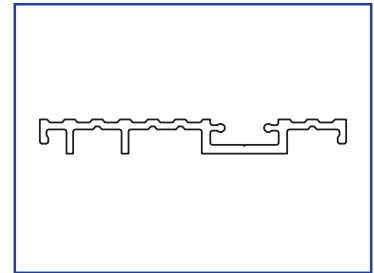
US01-0280-LLMF Threshold, Standard, UniSlide
