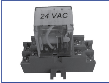
USREL24VAC Relay Kit, 24VAC, DPDT w/Base
