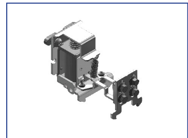
1011004 Lock, Electric, Fail-Safe, Telescopic (Shown)
