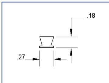
85-20-012 Felt Pile, Self Adhesive, 1/4" Back, BK
