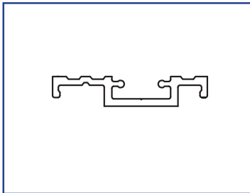
US01-0581-LLMF Threshold, Surface Applied Extension 2 5/8", Telescopic
