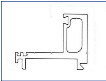
US01-1603-LLCL Impact Gutter, CL
