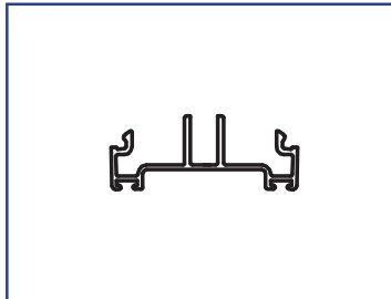
US01-0352-LLCL Plank Cap, FSL/FBO
