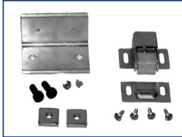
55-15-055 Mounting Kit, Nylatch, ICU (set of Two)
