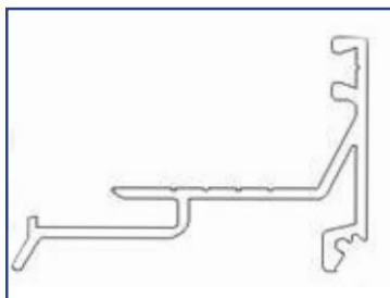
US01-1638-LLCL 1-1/4" Gutter, Clear
