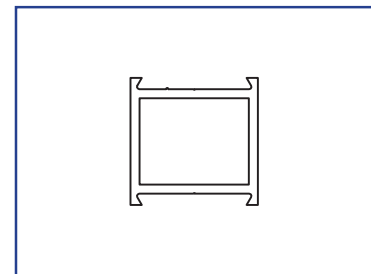
US01-0413-LLCL Horizontal Muntin, 1 3/4"
