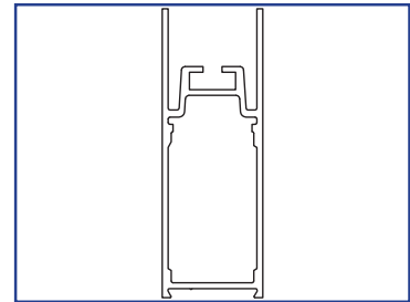
US01-0456-LLCL 5" Top Rail
