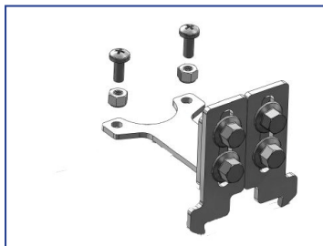
1010748 Electric Lock Bracket Assembly, Telescopic
