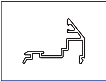
US01-0423-LLCL 1/4" Sloped Gutter
