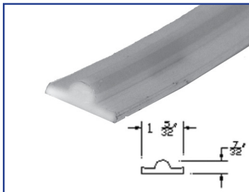
18-20-002 Track, C Series
