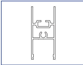
US01-0455-LLCL 2 3/16" Top Rail
