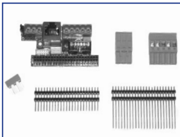
1003557 Safety Kit, EXU-SA ***Use with door mounted safety sensor and relay output for door/error indication.
