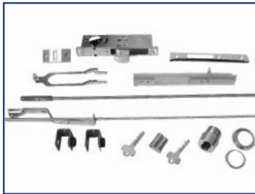
US05-0436-02 3-Pt Lock Assembly, Target, Exterior
