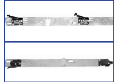
H21081 Switch, Back Check, Open Cut-off (Top)
