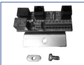
1011621 Unislide Mode Selec- tor Connection Board w/ cable ( Metal Bracket )
