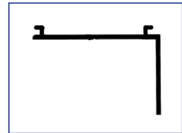
1008138-LLCL Mounting Angle, S/L, CL
