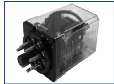
US5X826 Relay, 24VAC, DPDT, 8 Pin
