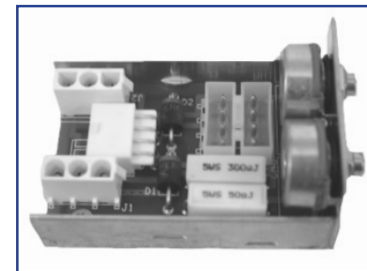
S516660 Control, Speed Close, Rebuilt
