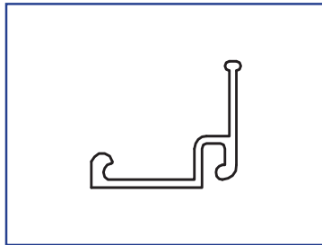
US01-0932-LLCL Redesigned 1/4" Snap, New
