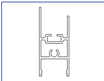
US01-0414-LLCL Active Leaf Bottom Rail, FBO
