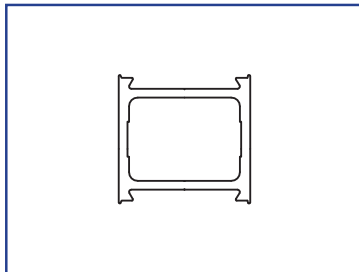
US01-0452-LLCL Vertical Muntin, Ready-Fold
