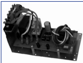
N4200102 Control, Swing "B", Hydraulic, Rebuilt
