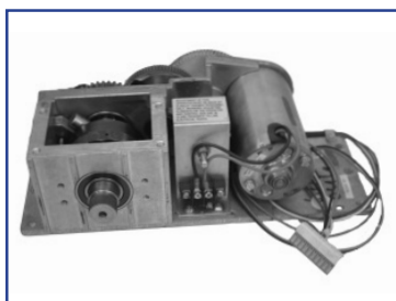
S1103791R Gearbox Motor, Outswing, LH, Rebuilt
