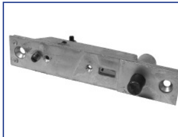
50-05-044 Pivot, Lock Pin, Retractable, Regular Duty
