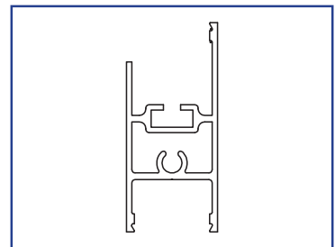
US01-0415-LLCL Side Lite Bottom Rail, FSL
