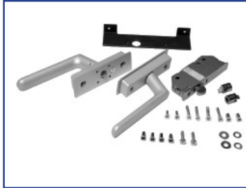
US15-0367-01 Positive Latching Kit, CL, ICU/CCU
