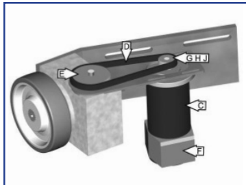
265022 Drive Unit Complete ( A ) (NOTE BRACKET LOCATION)
