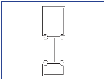
US01-0934-LLCL Redesigned Mullion Tube
