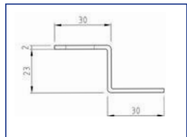
245834 Z Bracket, Ceiling
