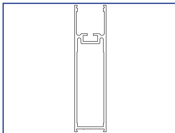
US01-0416-LLCL 7" Bottom Rail
