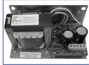
H3955 Power Supply, Slider, Linear, 2150/Control, Rebuilt
