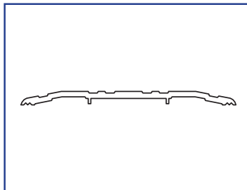
US01-0446-LLMF Threshold, 1/4" x 4"
