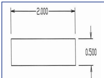
50-01-152 Crash Bar, 1/2" x 2", CL
