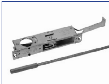
US08-0651-01 Lock Body, 31/32" (Includes Bottom Lock Rod)
