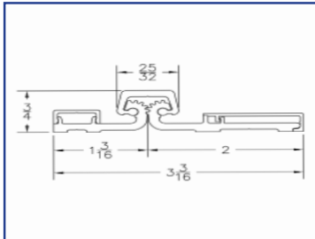
US78015783AL Full Surface Continuous Hinge, 83", CL
