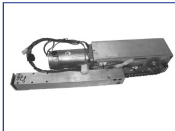
N3000LISSRCR Operator, Inswing, Square Shaft, SA, LH, Rebuilt
