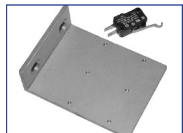
HC37331 Switch, Closed Monitor
