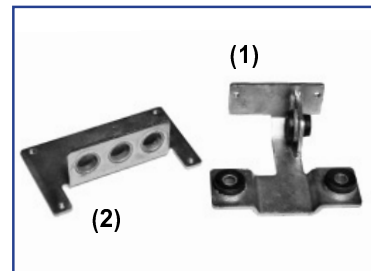
30-04-005 Mount, Operator, Hinge Side ( 1 )
