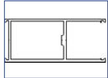
1012942-LLCL 4" Horizontal Rail, H4, CL
