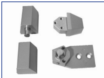
USJ27CL Kit, Pivot, Offset Top and Bottom, CL
