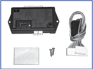
USORLM Lockout Relay, Optex 601 Sensor
