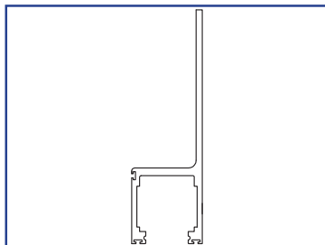
US01-0292-LLCL Carrier, Telescopic UniSlide **
