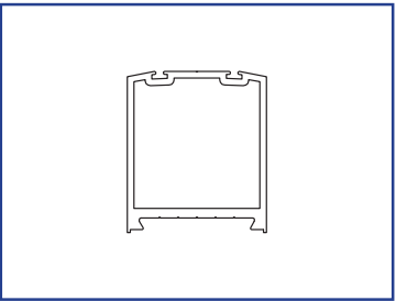
US01-1632-LLCL Narrow Stile Double Fuzz, Nose Rail, Standard Wall
