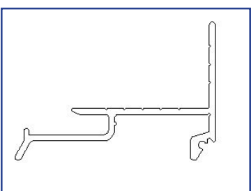
1009673-LLCL 1" Offset Gutter CL
