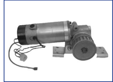
HC36751R Gearbox/Motor, 1/8 HP, Rebuilt, 6-7/8" long motor
