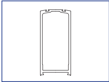
US01-0502-LLCL Medium Stile Double Fuzz, Nose Rail
