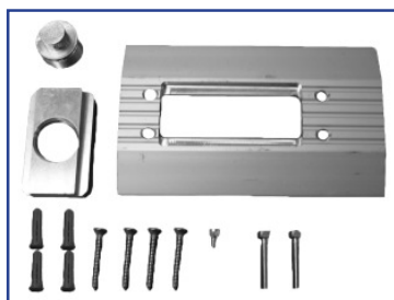
S3129031 Pivot, Bottom, Pkg., Adj., Taper, B/F
