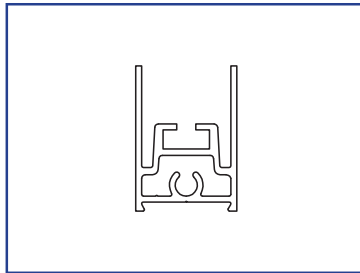
US01-0411-LLCL 2 1/2" Top Rail
