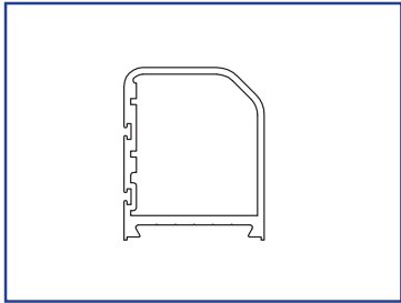
US01-1633-LLCL Narrow Stile Besam Rail, Standard Wall
