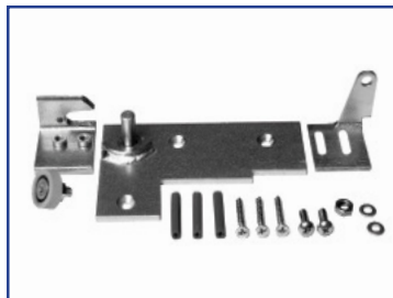
12-15-104 Pivot and Guide, A/L, RH, Kit (Shown)
