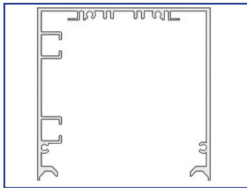
1008592-LLCL Extrusion, Head Box Beam, OHC, Bottom Load, SW200i, Clear
