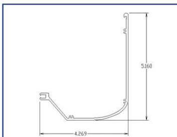
US01-1698-LLCL Auto Header Cover, CL
