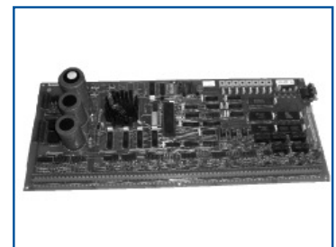
653677 Control, Main PCB, KDAC *(MCU1)
