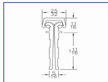
US78011283AL Concealed Leaf Continuous Hinge, 83", CL
