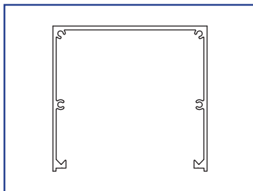
US01-0594-LLCL Bottom Load, Header, Swingmaster
