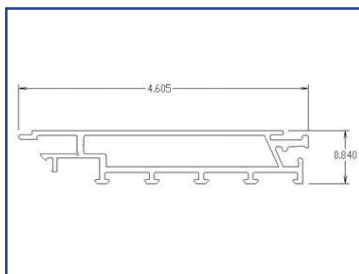
US01-1697-LLCL Auto Header Extension, CL
