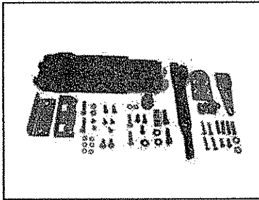
50-05-072 Closer, End Load, Light Duty, OHC
