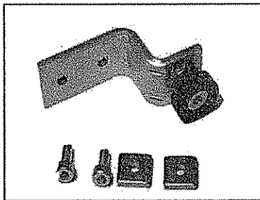
55-15-008 Roller Block Assembly, Bi-Way, ICU/CCU
