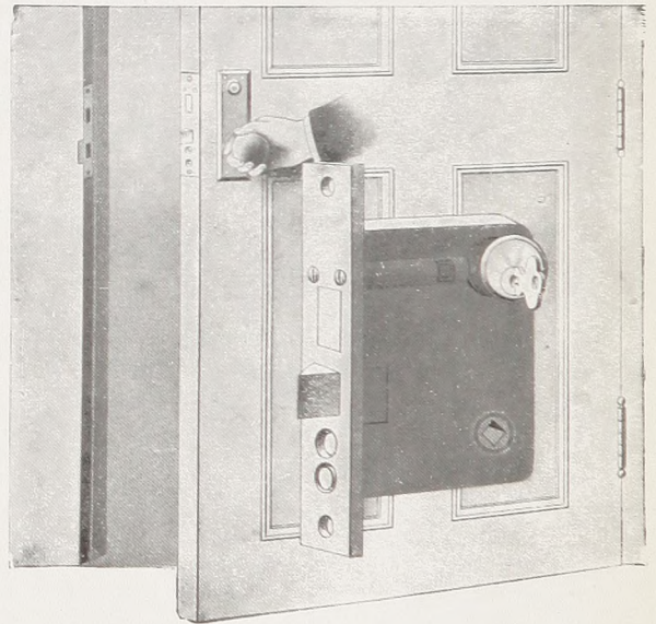
Right Hand Door opening out.
