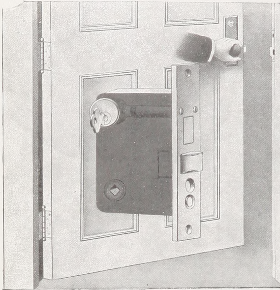
Left Hand Door opening in.
