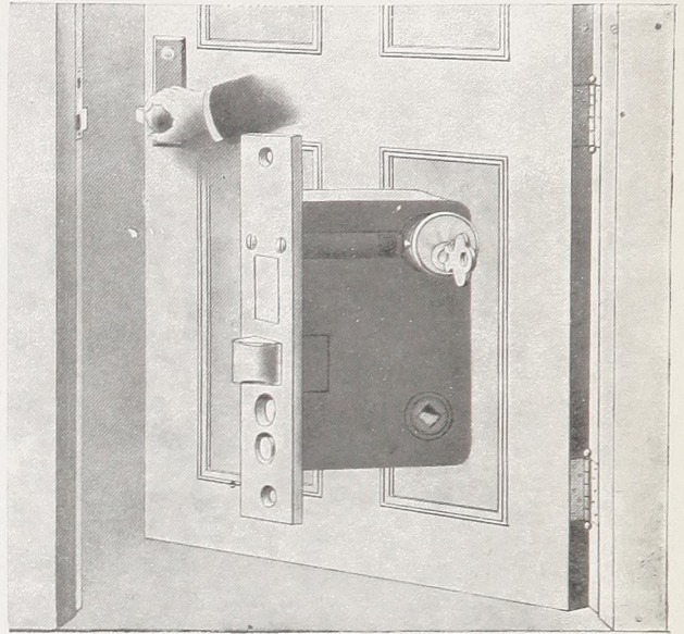
Right Hand Door opening in.
