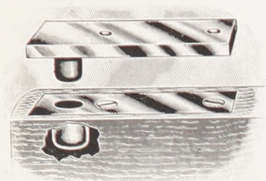
Top Pivot and Socket
