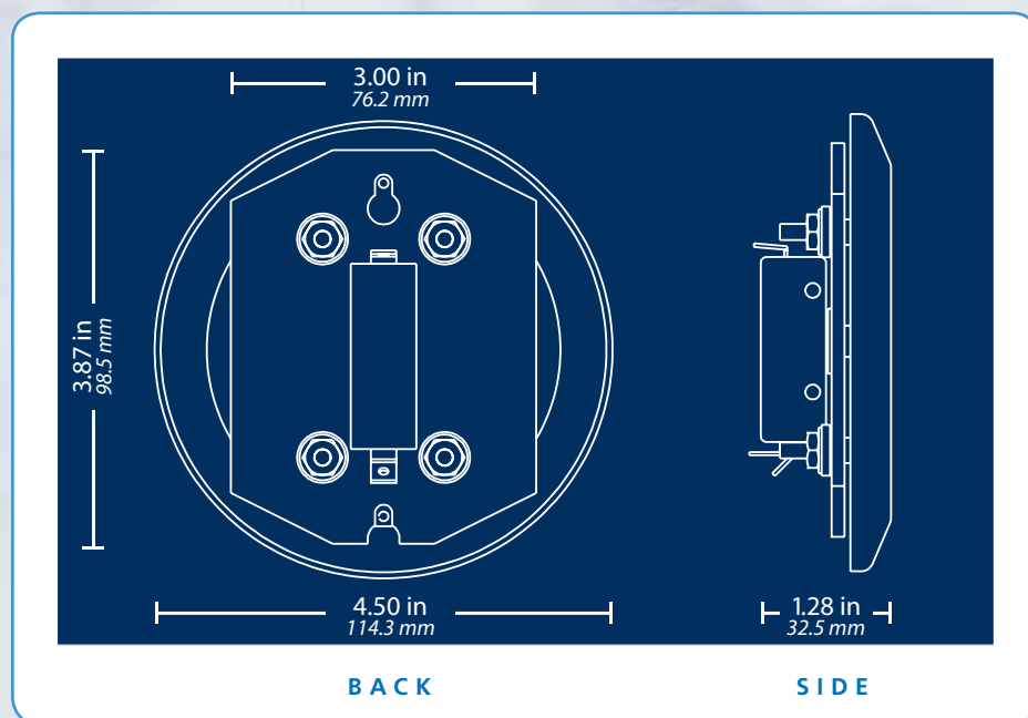
10ESCUTCHEON45 Stainless Steel Surface Mount
