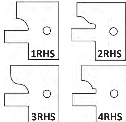
BELOW TIPS FIT THE STILE HEAD DESIGNED TO RUN COUNTER-CLOCKWISE WITH MATERIALS FACE-UP
