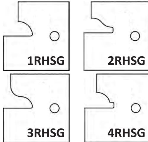
BELOW TIPS FIT THE STILE HEAD DESIGNED TO RUN COUNTER-CLOCKWISE WITH MATERIALS FACE-DOWN
