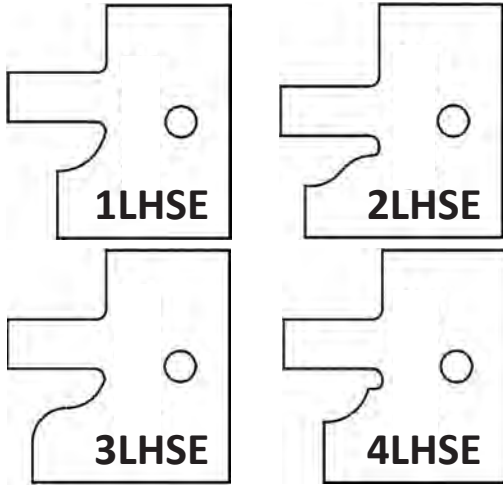
BELOW EASED EDGE TIPS FIT THE STILE HEAD DESIGNED TO RUN COUNTER-CLOCKWISE WITH MATERIALS FACE-DOWN
