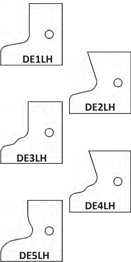
ABOVE 5 TIPS FIT A 3 WING HEAD DESIGNED TO RUN COUNTER-CLOCK WISE WITH MATERIALS FACE-DOWN
