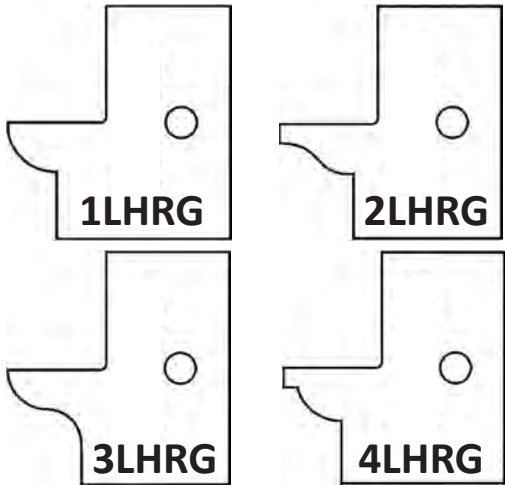
ABOVE TIPS FIT THE RAIL HEAD DESIGNED TO RUN COUNTER-CLOCKWISE WITH MATERIALS FACE-DOWN
