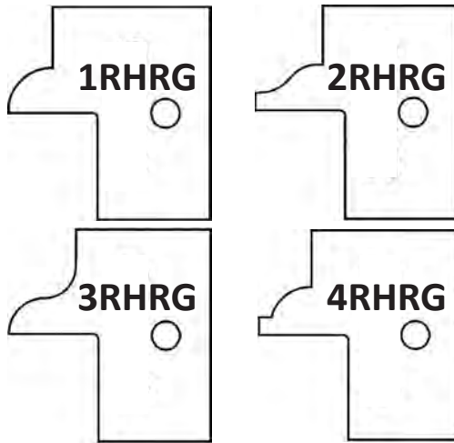
ABOVE TIPS FIT THE RAIL HEAD DESIGNED TO RUN COUNTER-CLOCKWISE WITH MATERIALS FACE-DOWN
