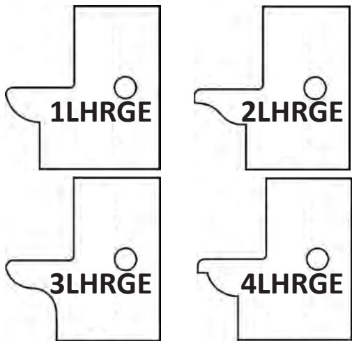
ABOVE EASED EDGE TIPS FIT THE RAIL HEAD DESIGNED TO RUN COUNTER-CLOCKWISE WITH MATERIALS FACE-DOWN
