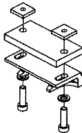
Carrier US05-1609-16 No Finish
