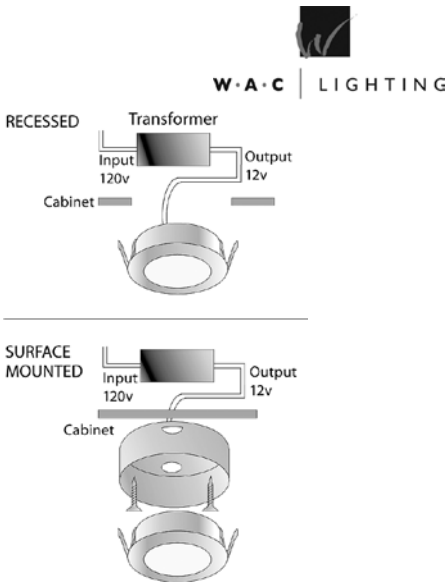
INSTALLATION DIAGRAMS Page J-46 Halogen Diagram H
