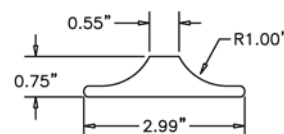
"T" Moulding Middle Piece
