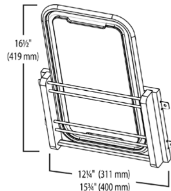
Door Mounting Brackets provide 5" of Adjustment
