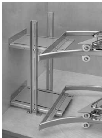
Adjustable Back Bracket
