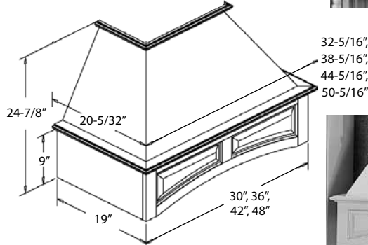
B - ARCHED RANGE WOOD
