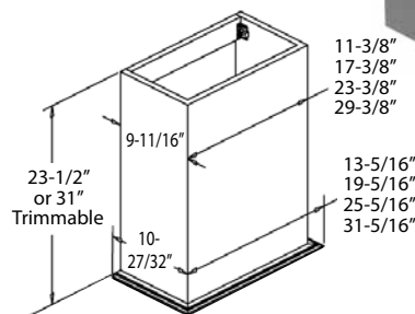
C - CUT-TO-SIZE CHIMNEY
