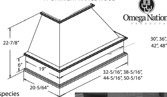
A - STRAIGHT RANGE WOOD
