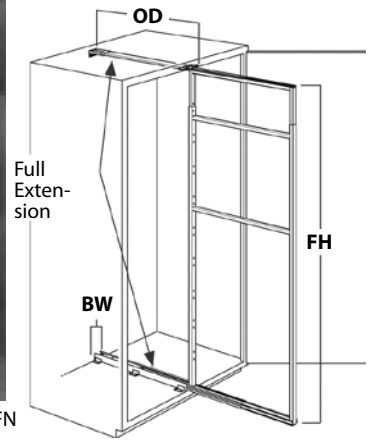
A - FYBP51875CM-W Center Mount Pantry Roll-Out Frame
