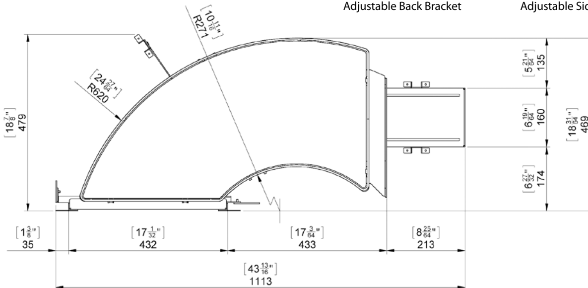
Adjustable Back Bracket
