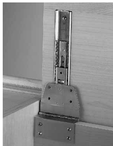
Assembly
