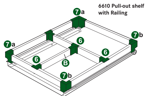
Front railing clip Dowelled
