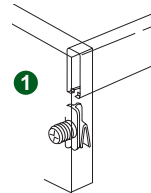
Back railing clip Screw-on
