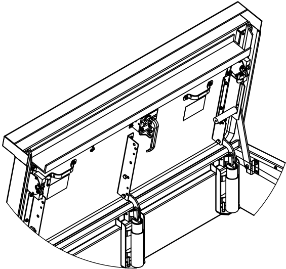
FACTORY INSTALLED VIEW
