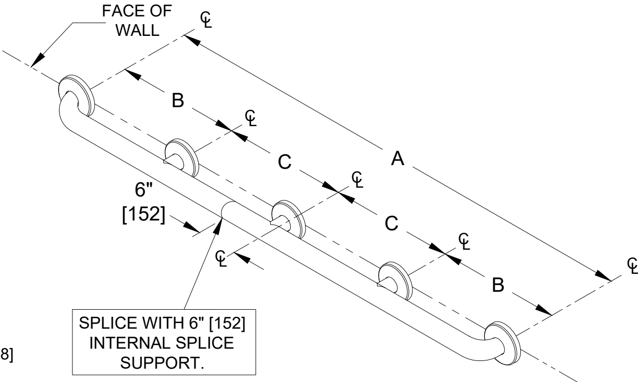
ISOMETRIC
