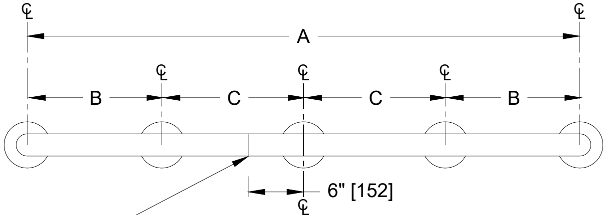
FRONT VIEW
