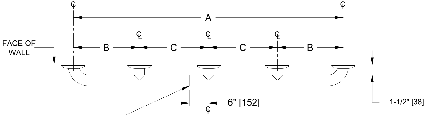
TOP VIEW
