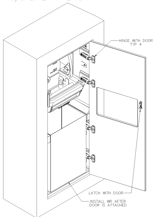
BREAKOUT VIEW FWD/CABINET INTERIOR
