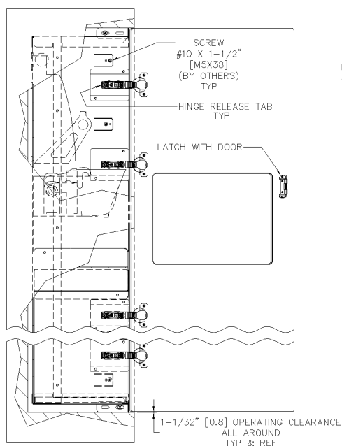
BREAKOUT VIEW FWD/CABINET INTERIOR
