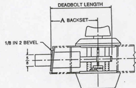
DRIVE-IN DEADBOLT SHOWN
