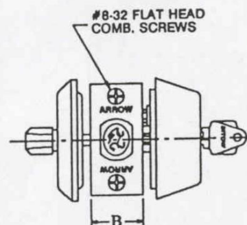
STRAIGHT FRONT SHOWN
