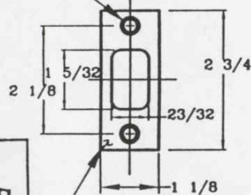
346 STRIKE (FOR METAL JAMB) APPLICATION
