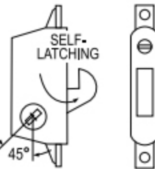
MS1847-11 LATCH
