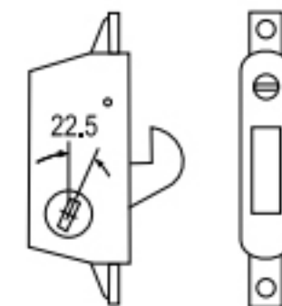
MS1847-09 LOCK
