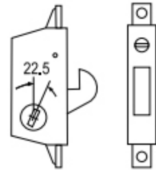
MS1847-10 LOCK
