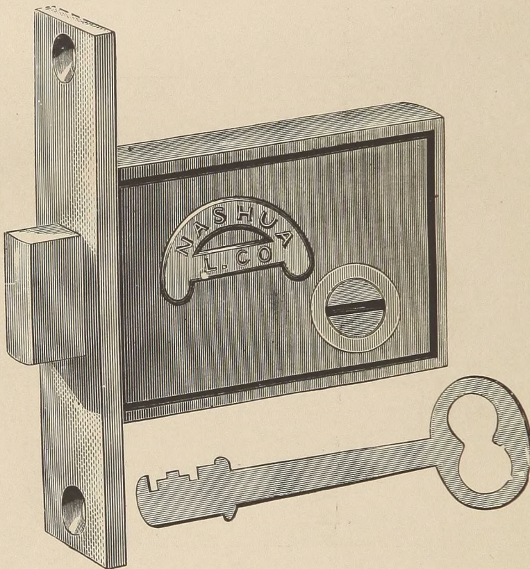
Full Size Cut of No. 359.
