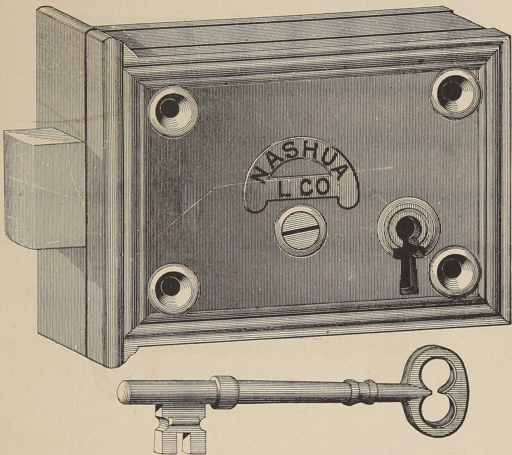
Full Size Cut of Nos. 510 and 511.
