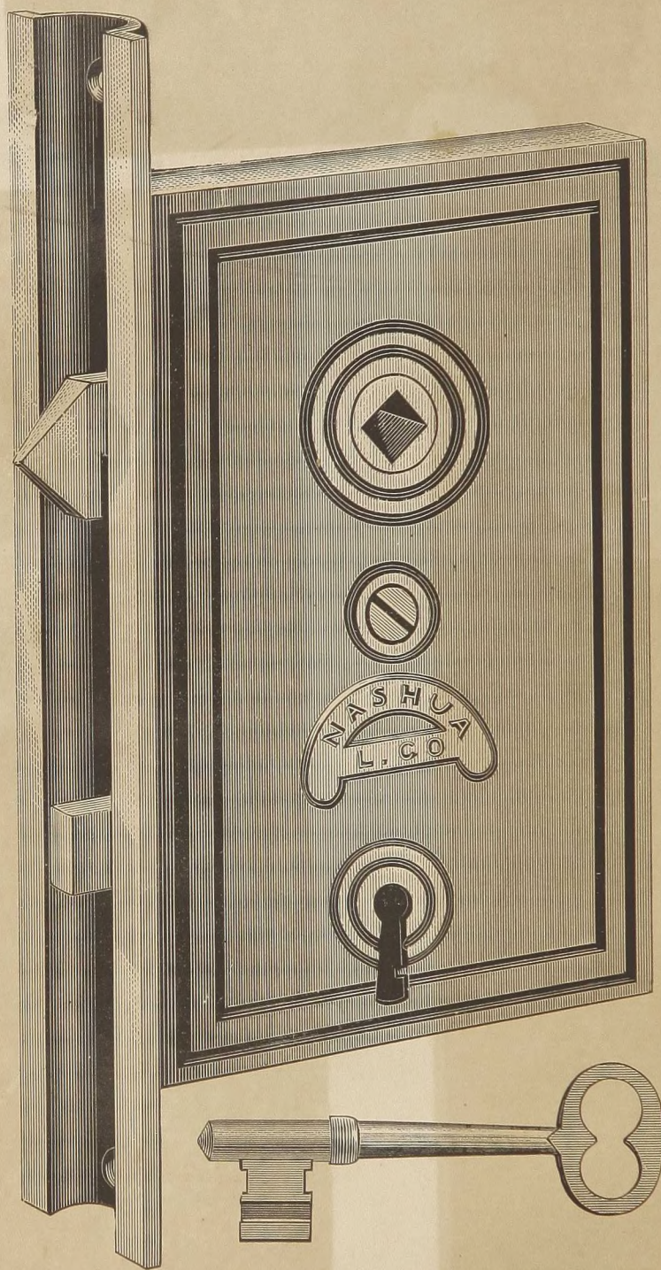
Full Size Cut of No. 141. For description, see opposite page.
