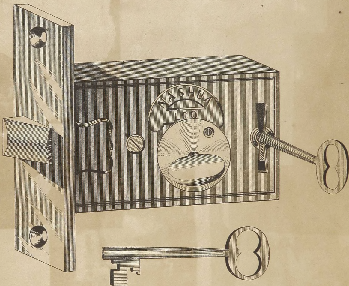
Full Size Cut of No. 85 1-2.
