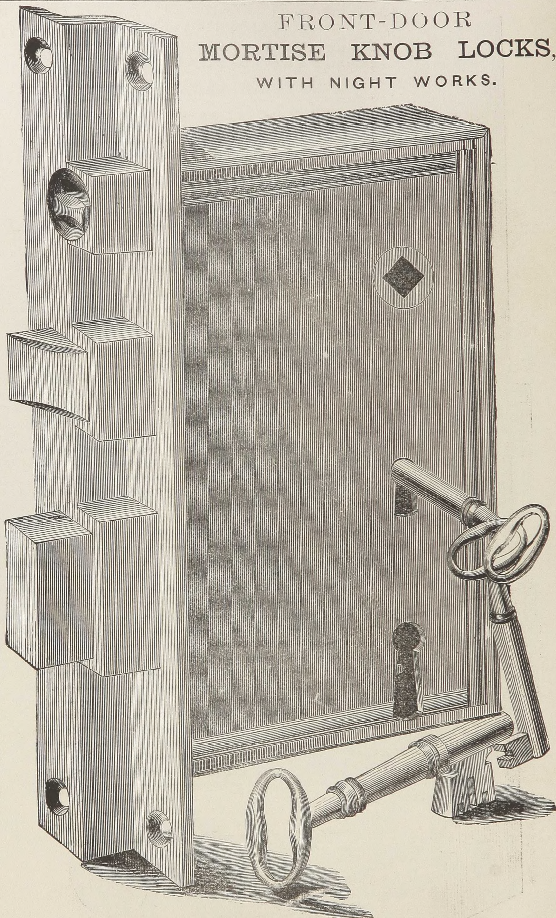
No. 138.—Size, 6\frac{1}{4} \times 4\frac{1}{2} INCHES.—Description on page 24.)
