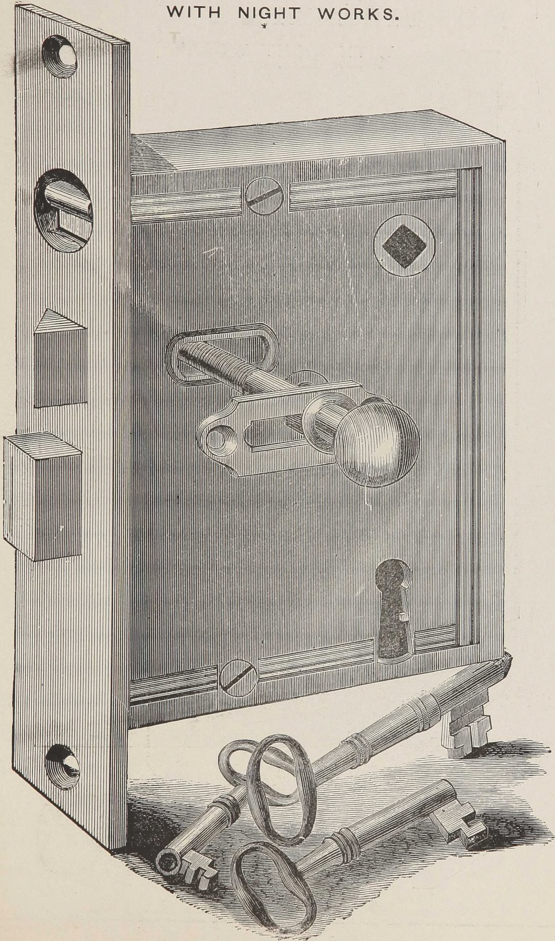
No. 135.—Size, 5\frac{1}{2} \times 4 INCHES.—(Description on page 24.)
