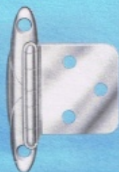
NO. 551 SEMI-CONCEALED HINGE FOR OVERLAY DOORS No Inset. Length of barrel 1\frac{1}{2} " Length of Pad 1\frac{3}{8} " Pat. No. D-182,889 Canadian Pat. No. RD1957
