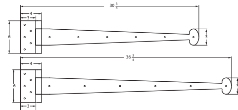
Dummy Strap- 30" & 36"
