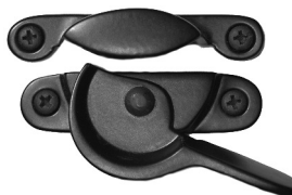
AK8BP 2-1/8" ctr-ctr - Catch 2" ctr-ctr - Latch
