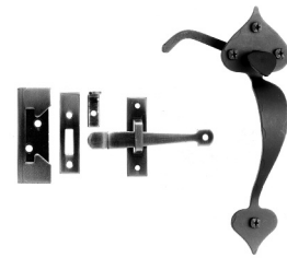
AT5BR: Reverse bevel/closet door. (handle on room side or exterior of storm door) 8-1/2" x 2-1/4" proj. 1-1/2" RSBBR: Rough handle
