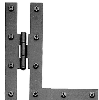
AH6BQ (4") Flush > 30-40 lbs. AH8BQ (7") Flush > 70-80 lbs.
