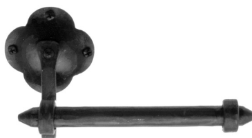
IBKBP Height: 3-1/4" Length: 8-1/4" Proj. 3-3/4"
