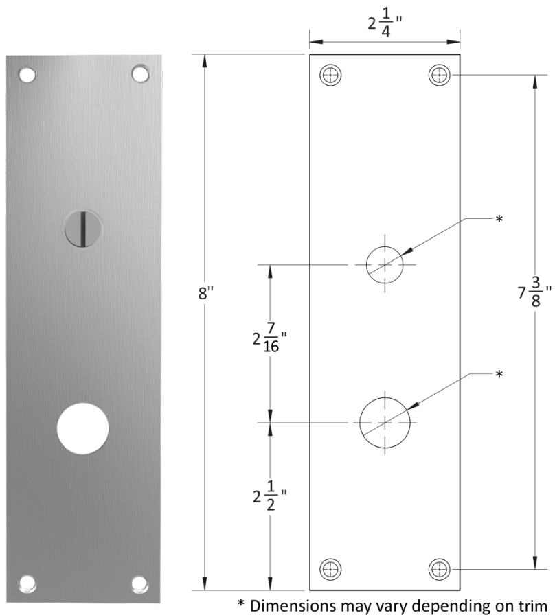
1E-E Emergency Coin Release
