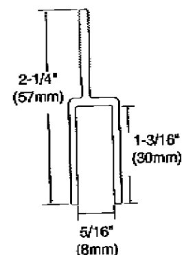
Top Hanger for 1/4" (6mm) Glass
