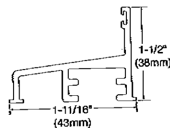
Bottom Track for 3/8" (10mm) or 1/4" (6mm) Glass
