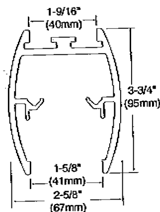
Header for 3/8" (10mm) Glass or 1/4" (6mm) Glass
