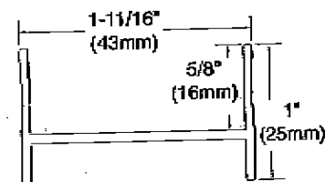
Side Jamb for 3/8" (10mm) or 1/4" (6mm) Glass
