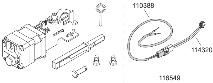
HD-QEL (Hex Dogging QEL) Kit (Panic Only) - 958002
