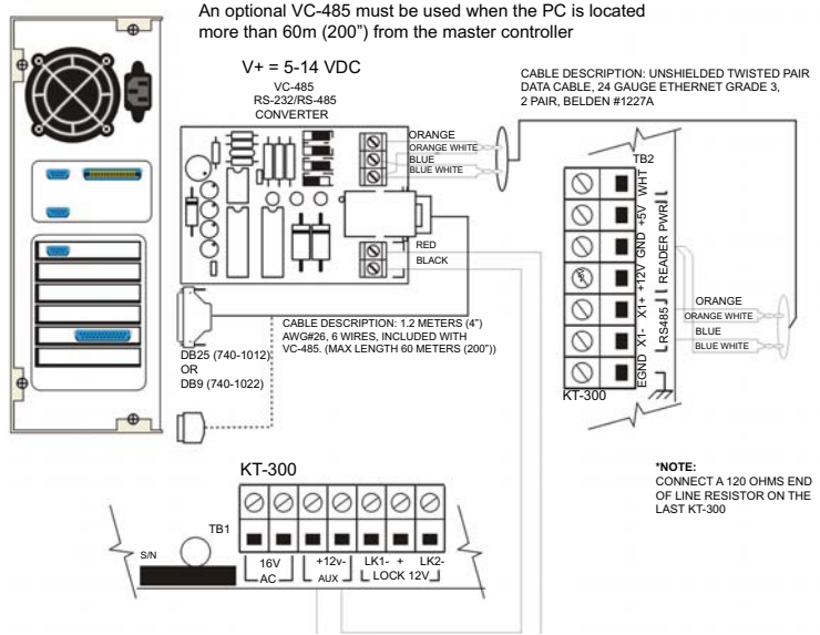
RS-485 WITH VC-485
