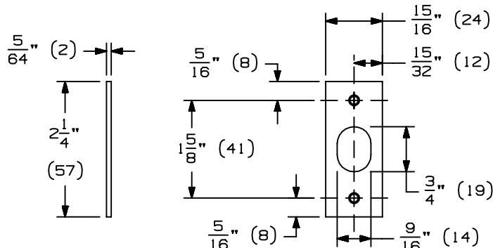
STRIKE
